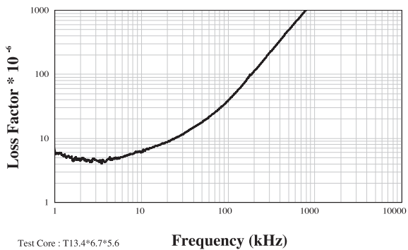
Loss Factor V.S. Frequency
