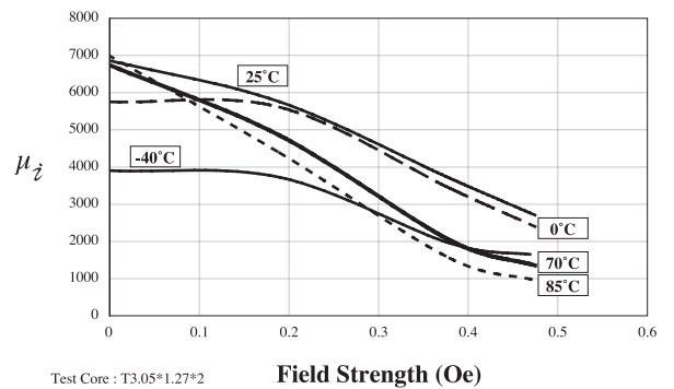
Initial Permeability V.S. Field Strength
