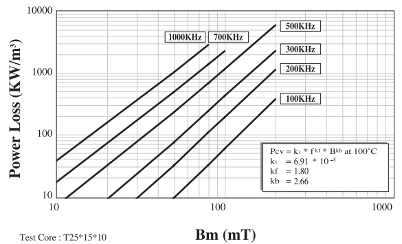
Power Loss V.S. Temperature/Flux Density/Frequency
