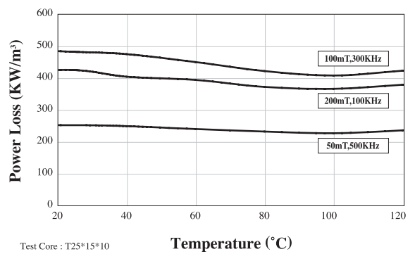
Power Loss V.S. Temperature
