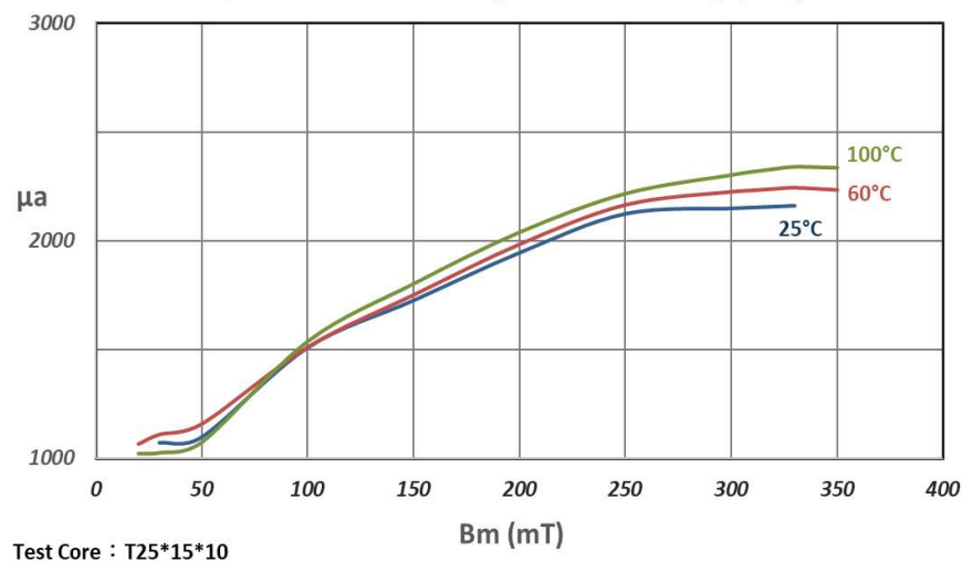
Amplitude Permeability vs Flux Density (Bm)
