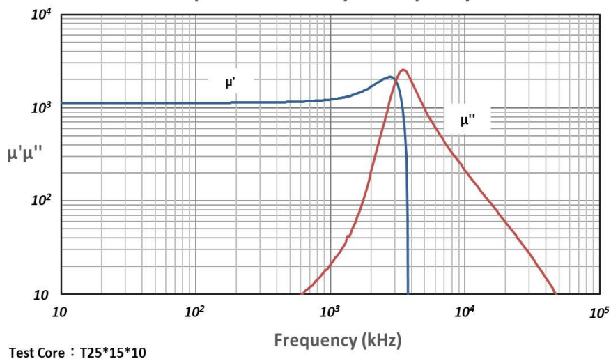
Complex Permeability vs Frequency
